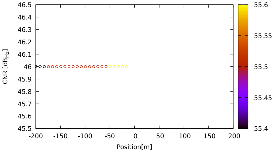
CNR vs position for E05 (E5) on LeicaGS15 - DOY 262 jam. 3
