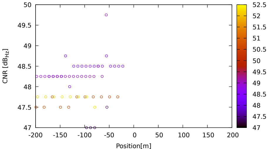
CNR vs position for E05 (E5a) on LeicaGS15 - DOY 262 jam. 2
