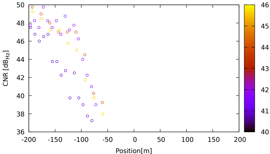
CNR vs position for E05 (E5b) on LeicaGS15 - DOY 262 jam. 1
