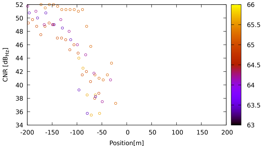
CNR vs position for E09 (E1) on LeicaGS15 - DOY 262 jam. 2
