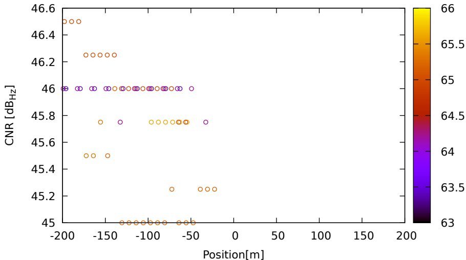
CNR vs position for E09 (E5) on LeicaGS15 - DOY 262 jam. 2
