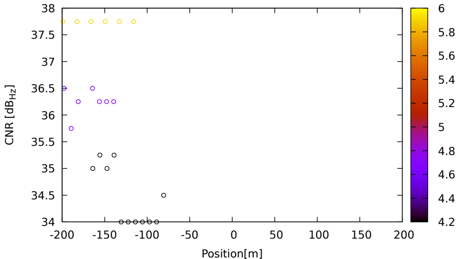
CNR vs position for E15 (E5) on LeicaGS15 - DOY 262 jam. 2
