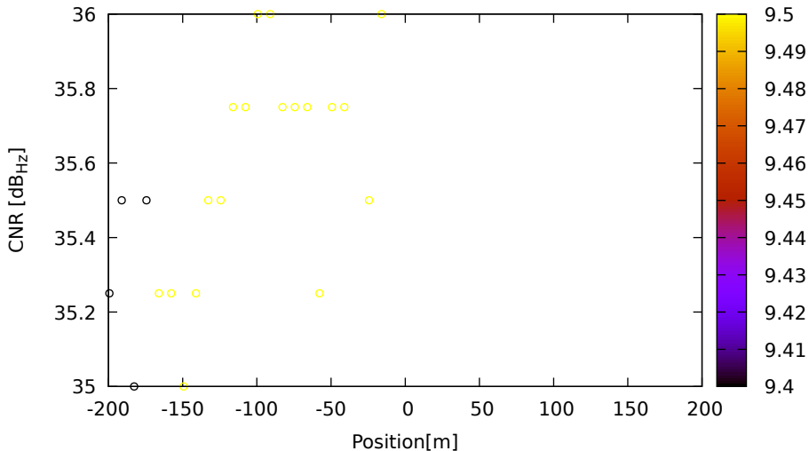
CNR vs position for E15 (E5) on LeicaGS15 - DOY 262 jam. 3
