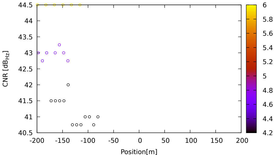
CNR vs position for E15 (E5b) on LeicaGS15 - DOY 262 jam. 2
