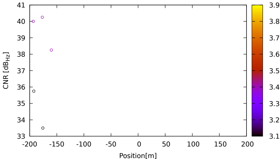
CNR vs position for E27 (E1) on LeicaGS15 - DOY 262 jam. 1
