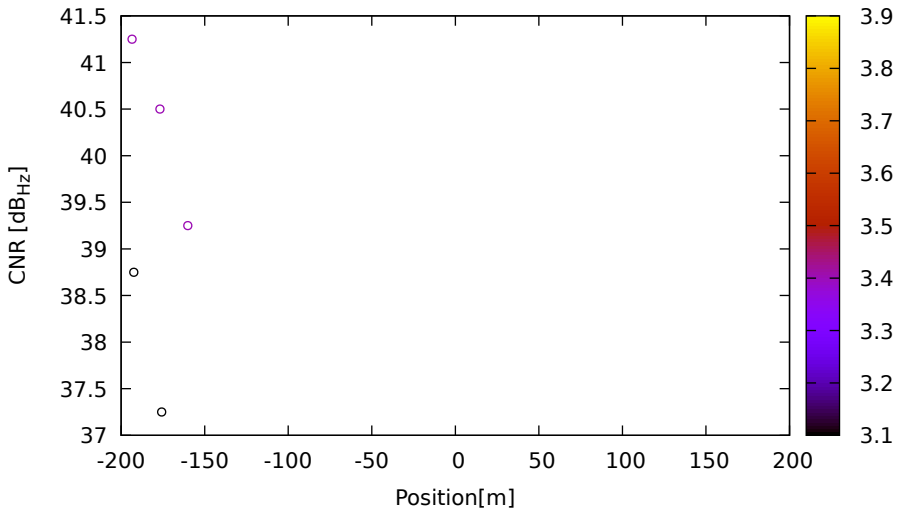
CNR vs position for E27 (E5b) on LeicaGS15 - DOY 262 jam. 1
