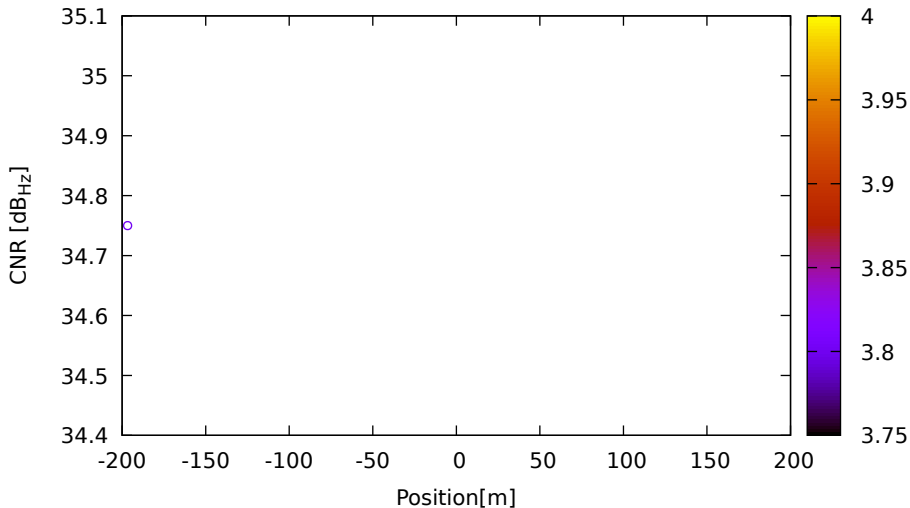
CNR vs position for E30 (E1) on LeicaGS15 - DOY 262 jam. 1
