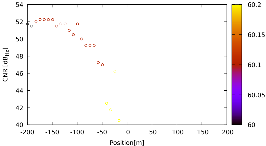
CNR vs position for E34 (E1) on LeicaGS15 - DOY 262 jam. 3
