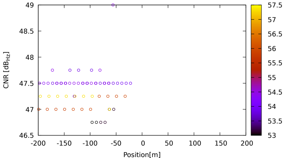
CNR vs position for E34 (E5a) on LeicaGS15 - DOY 262 jam. 2
