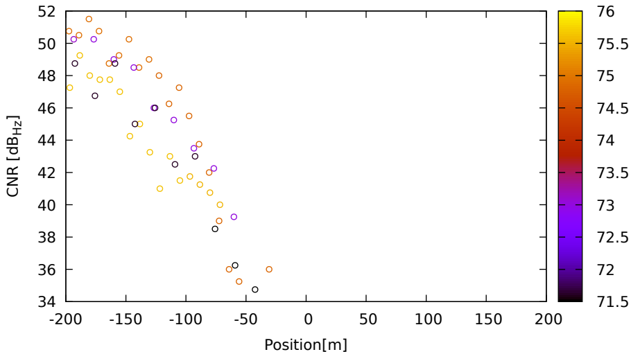
CNR vs position for E36 (E1) on LeicaGS15 - DOY 262 jam. 1
