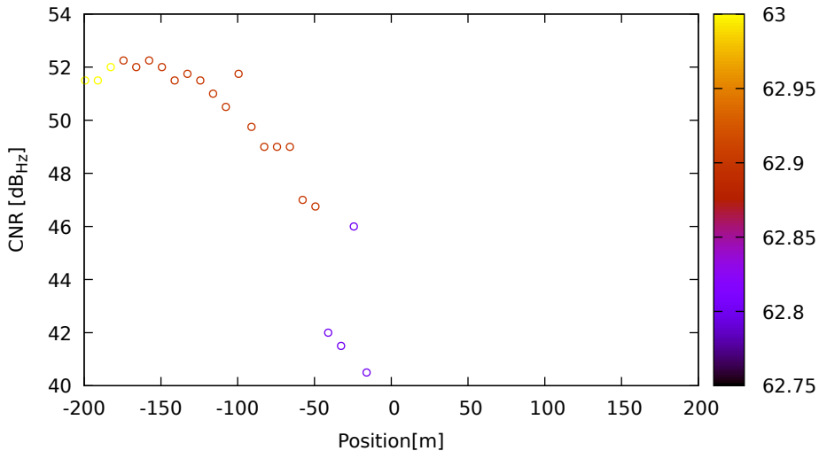
CNR vs position for E36 (E1) on LeicaGS15 - DOY 262 jam. 3
