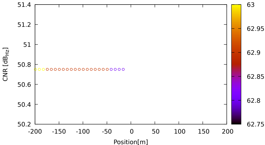
CNR vs position for E36 (E5b) on LeicaGS15 - DOY 262 jam. 3
