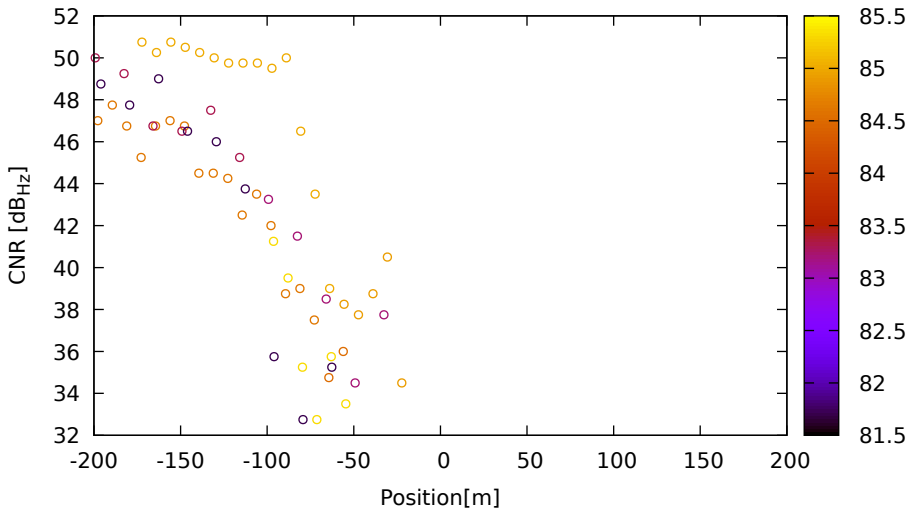
CNR vs position for G01 (L1) on LeicaGS15 - DOY 262 jam. 2
