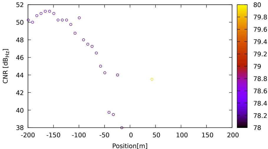
CNR vs position for G01 (L2) on LeicaGS15 - DOY 262 jam. 3
