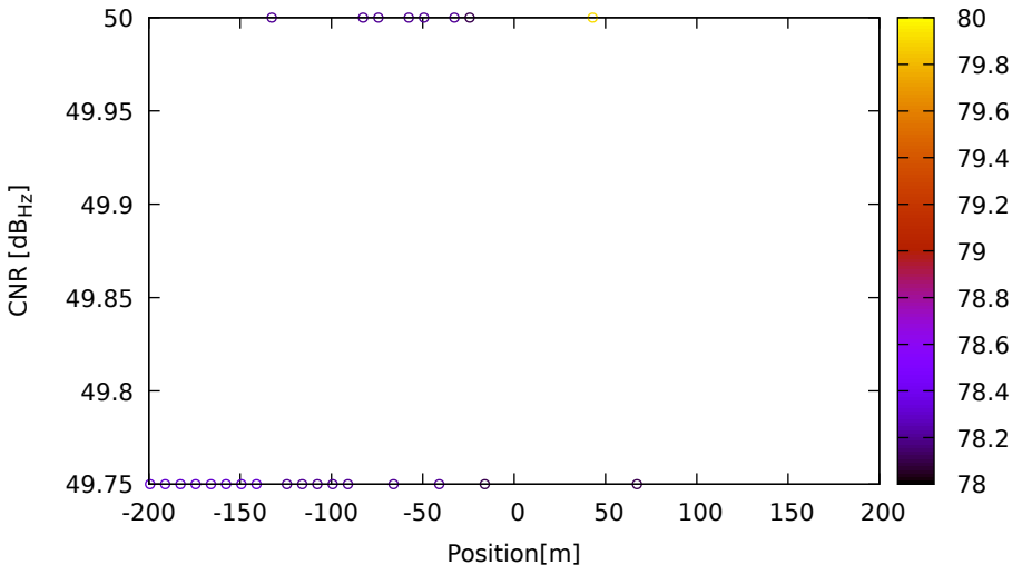
CNR vs position for G01 (L5) on LeicaGS15 - DOY 262 jam. 3
