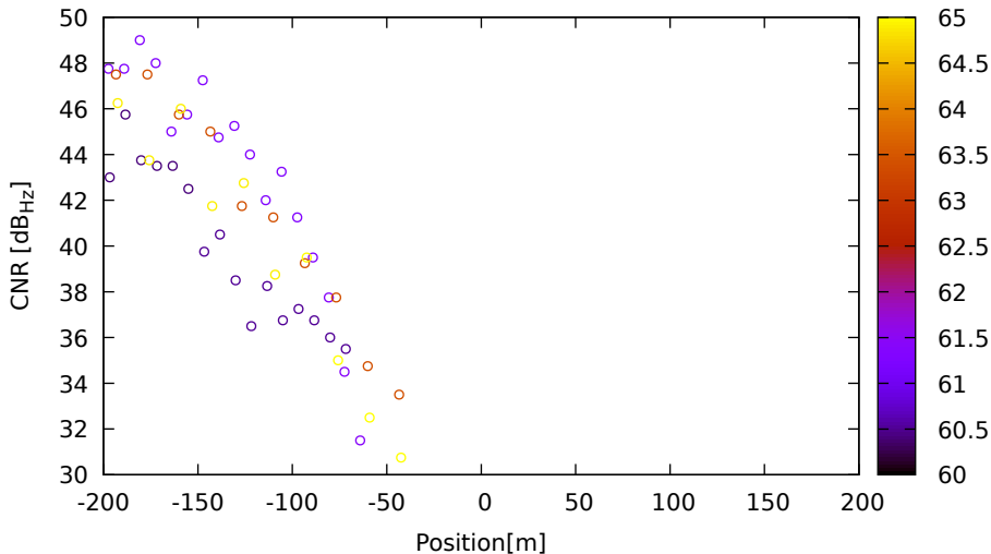
CNR vs position for G03 (L1) on LeicaGS15 - DOY 262 jam. 1
