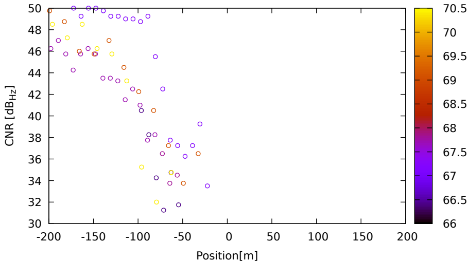
CNR vs position for G03 (L1) on LeicaGS15 - DOY 262 jam. 2
