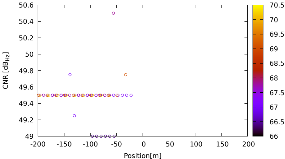
CNR vs position for G03 (L5) on LeicaGS15 - DOY 262 jam. 2
