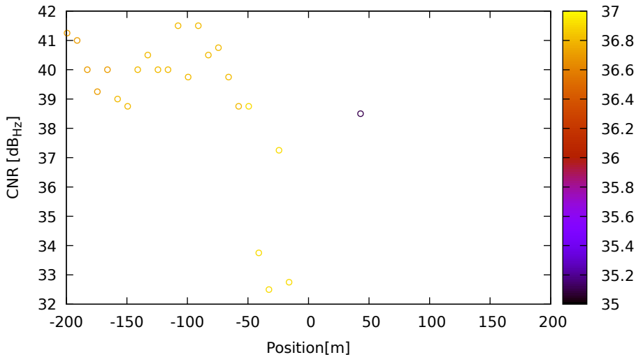
CNR vs position for G04 (L2) on LeicaGS15 - DOY 262 jam. 3
