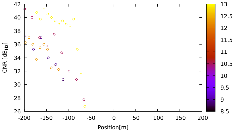
CNR vs position for G08 (L1) on LeicaGS15 - DOY 262 jam. 2
