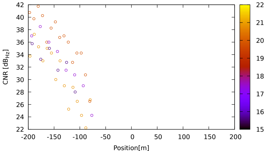
CNR vs position for G08 (L2) on LeicaGS15 - DOY 262 jam. 1
