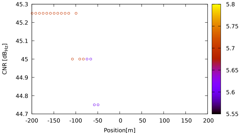
CNR vs position for G08 (L5) on LeicaGS15 - DOY 262 jam. 3
