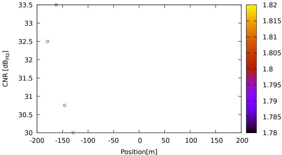
CNR vs position for G09 (L2) on LeicaGS15 - DOY 262 jam. 2
