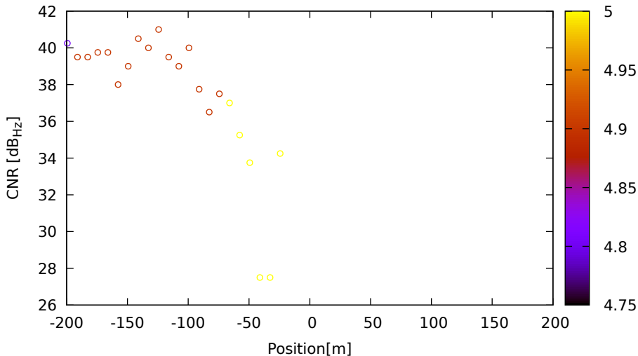
CNR vs position for G09 (L2) on LeicaGS15 - DOY 262 jam. 3
