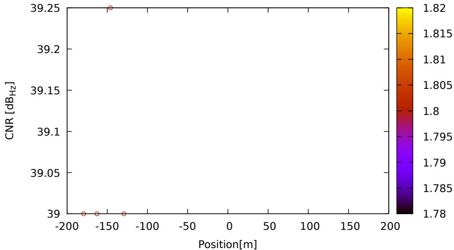
CNR vs position for G09 (L5) on LeicaGS15 - DOY 262 jam. 2
