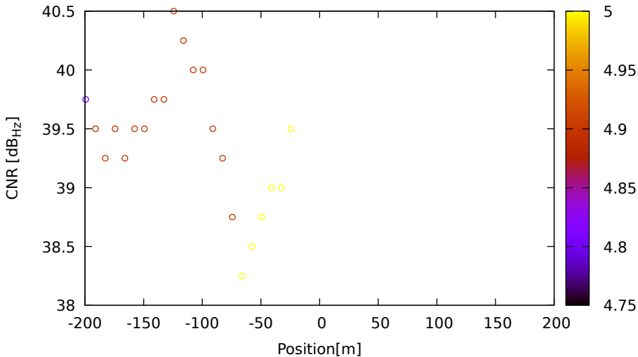
CNR vs position for G09 (L5) on LeicaGS15 - DOY 262 jam. 3
