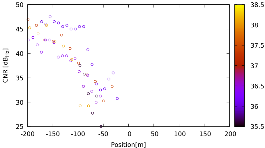
CNR vs position for G17 (L2) on LeicaGS15 - DOY 262 jam. 2
