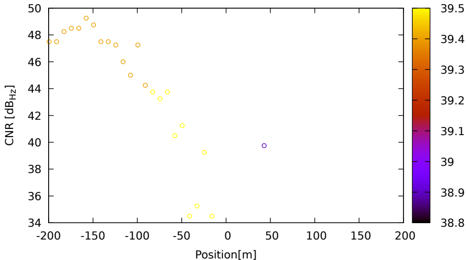
CNR vs position for G17 (L2) on LeicaGS15 - DOY 262 jam. 3
