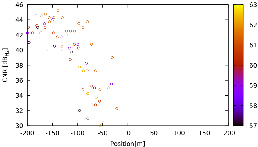
CNR vs position for G21 (L2) on LeicaGS15 - DOY 262 jam. 2
