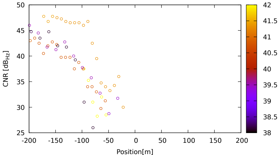
CNR vs position for G22 (L1) on LeicaGS15 - DOY 262 jam. 2
