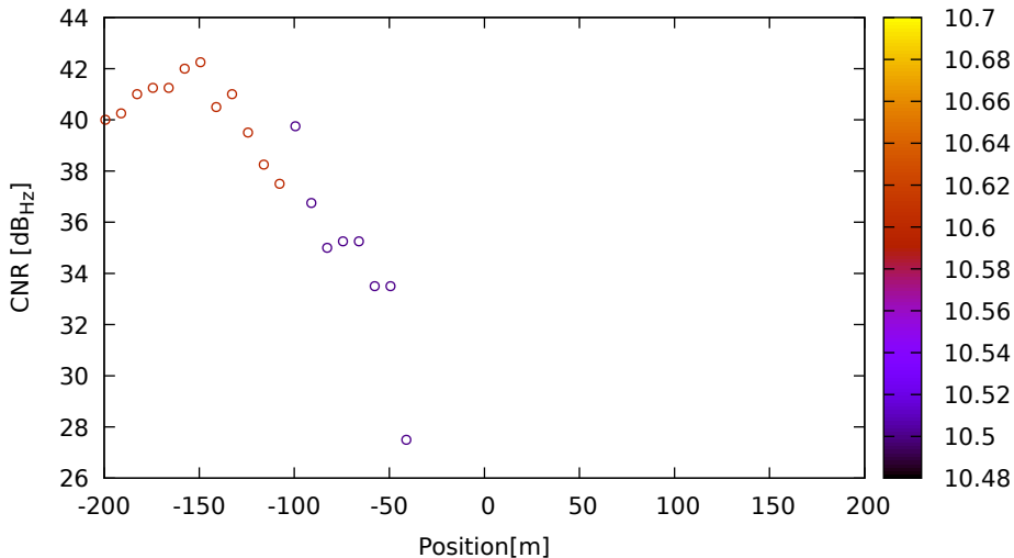
CNR vs position for G32 (L1) on LeicaGS15 - DOY 262 jam. 3
