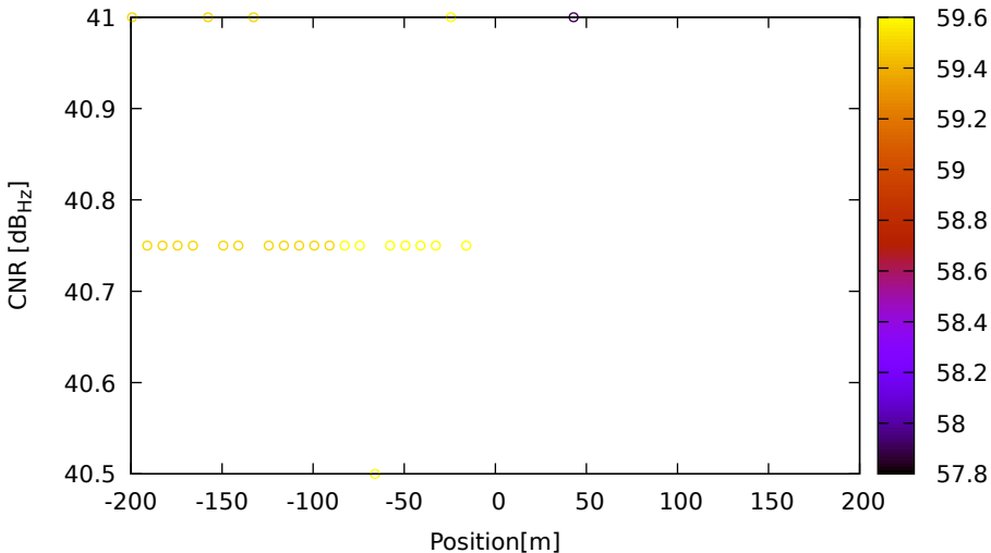
CNR vs position for R01 (G2) on LeicaGS15 - DOY 262 jam. 3
