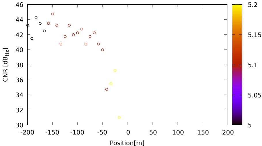
CNR vs position for R02 (G1) on LeicaGS15 - DOY 262 jam. 3
