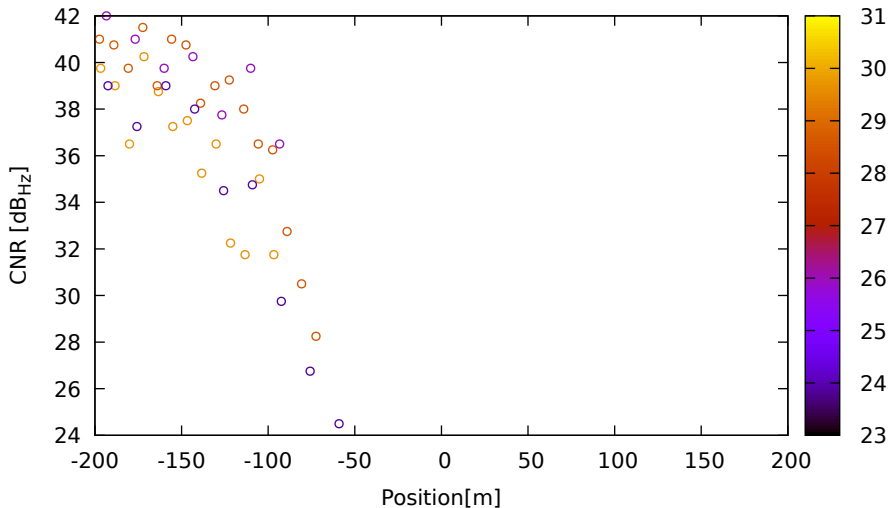
CNR vs position for R07 (G2) on LeicaGS15 - DOY 262 jam. 1
