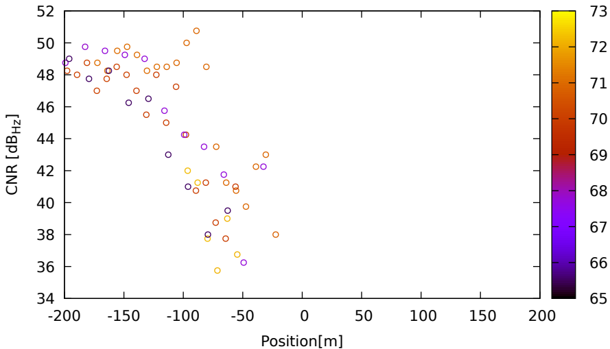
CNR vs position for R08 (G1) on LeicaGS15 - DOY 262 jam. 2
