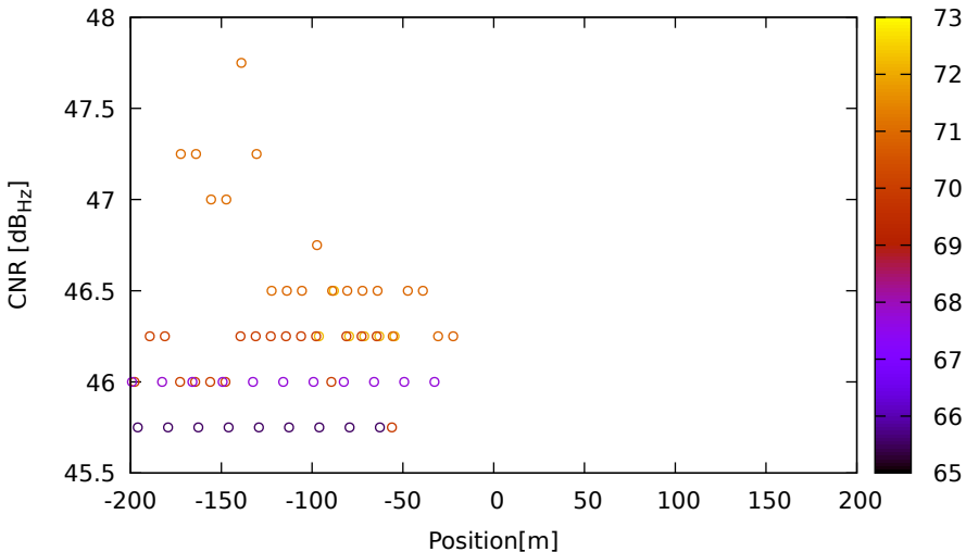
CNR vs position for R08 (G2) on LeicaGS15 - DOY 262 jam. 2
