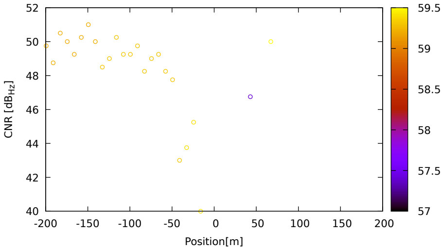
CNR vs position for R24 (G1) on LeicaGS15 - DOY 262 jam. 3
