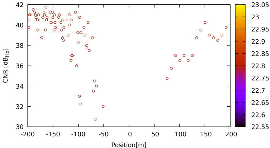
CNR vs position for C05 (B1) on LeicaGS18 - DOY 262 jam. 2
