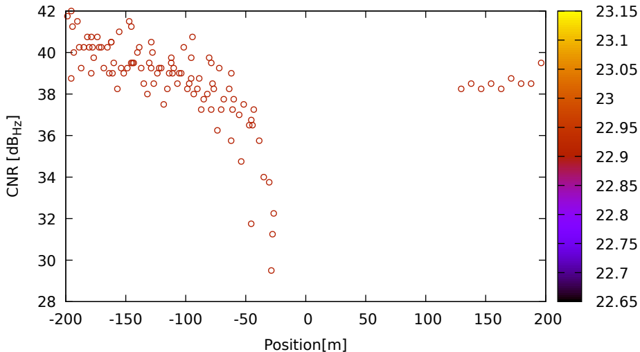
CNR vs position for C05 (B2) on LeicaGS18 - DOY 262 jam. 1
