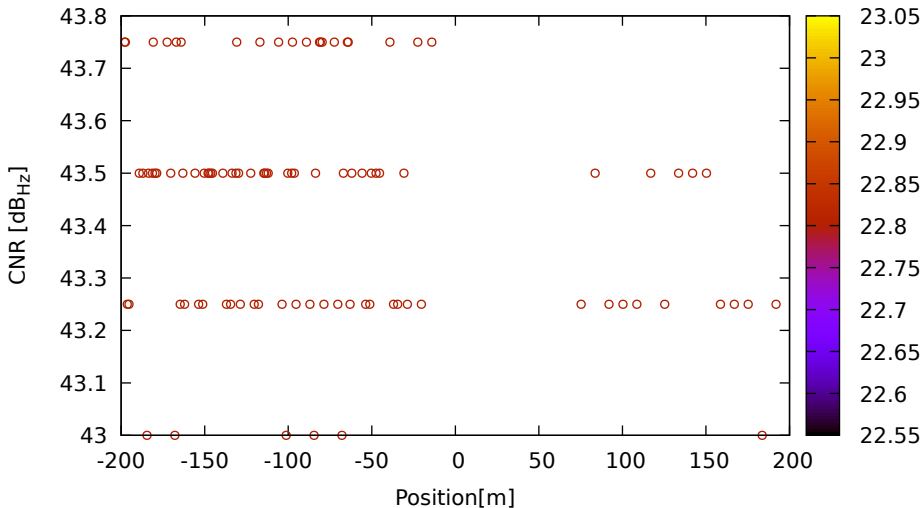
CNR vs position for C05 (B2) on LeicaGS18 - DOY 262 jam. 2
