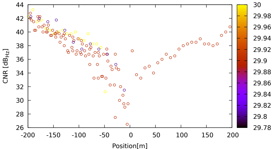
CNR vs position for C06 (B1) on LeicaGS18 - DOY 262 jam. 1
