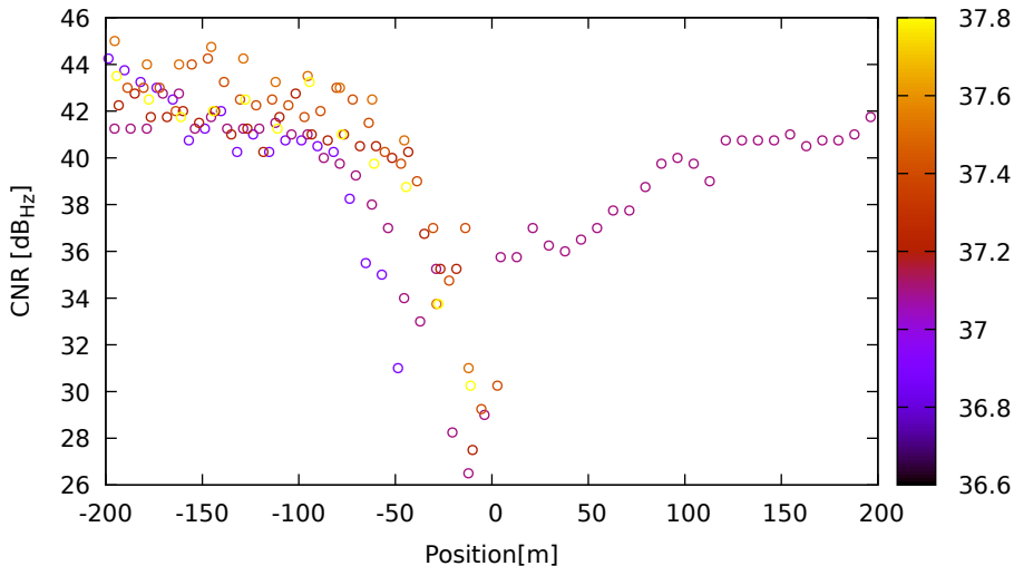
CNR vs position for C09 (B2) on LeicaGS18 - DOY 262 jam. 1
