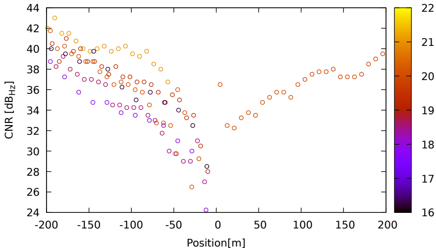
CNR vs position for C11 (B1) on LeicaGS18 - DOY 262 jam. 1
