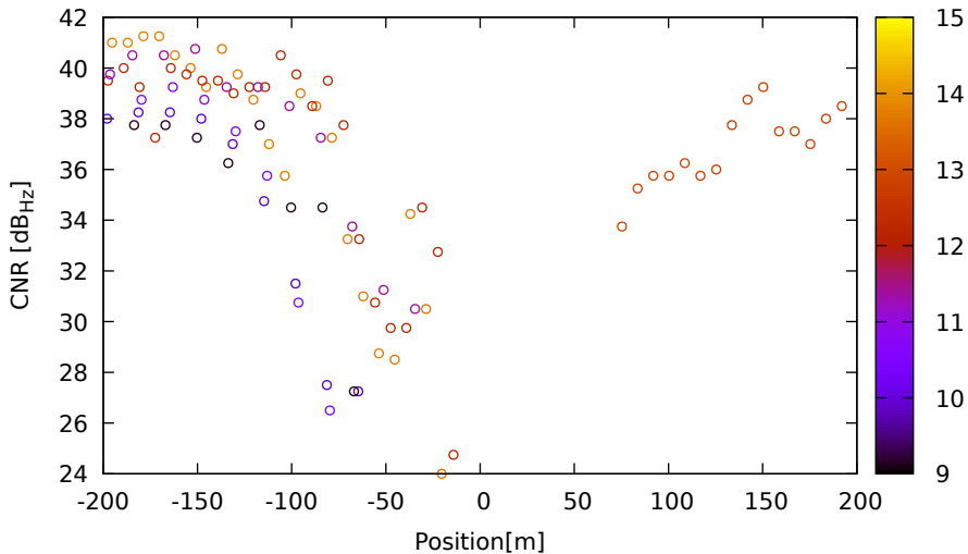
CNR vs position for C11 (B1) on LeicaGS18 - DOY 262 jam. 2
