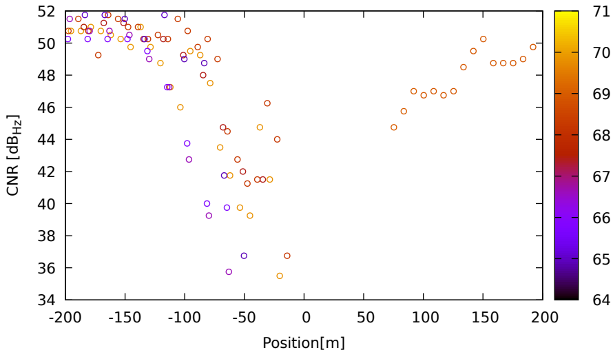
CNR vs position for C14 (B1) on LeicaGS18 - DOY 262 jam. 2
