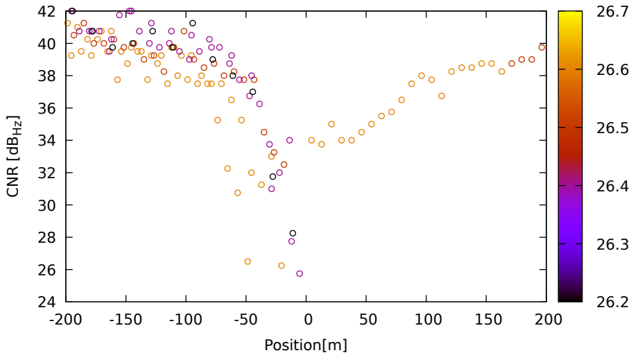
CNR vs position for C16 (B2) on LeicaGS18 - DOY 262 jam. 1
